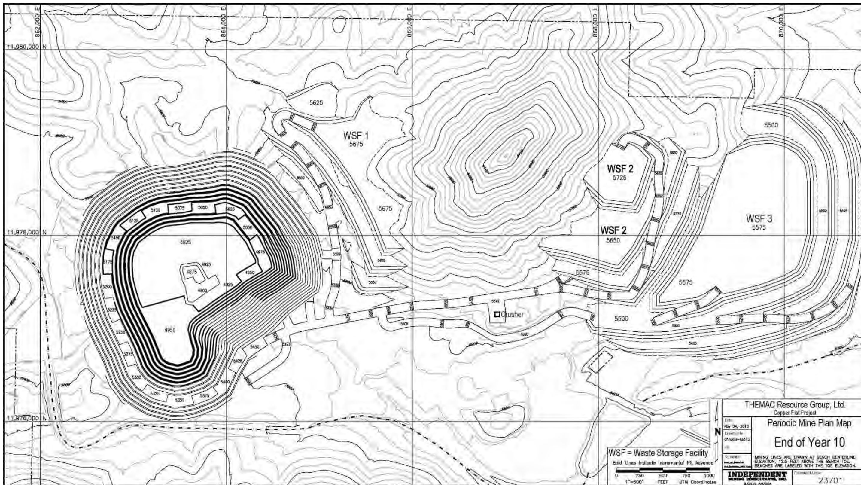
Figure 16-12: Periodic Mine Plan Map – End of Year 10
