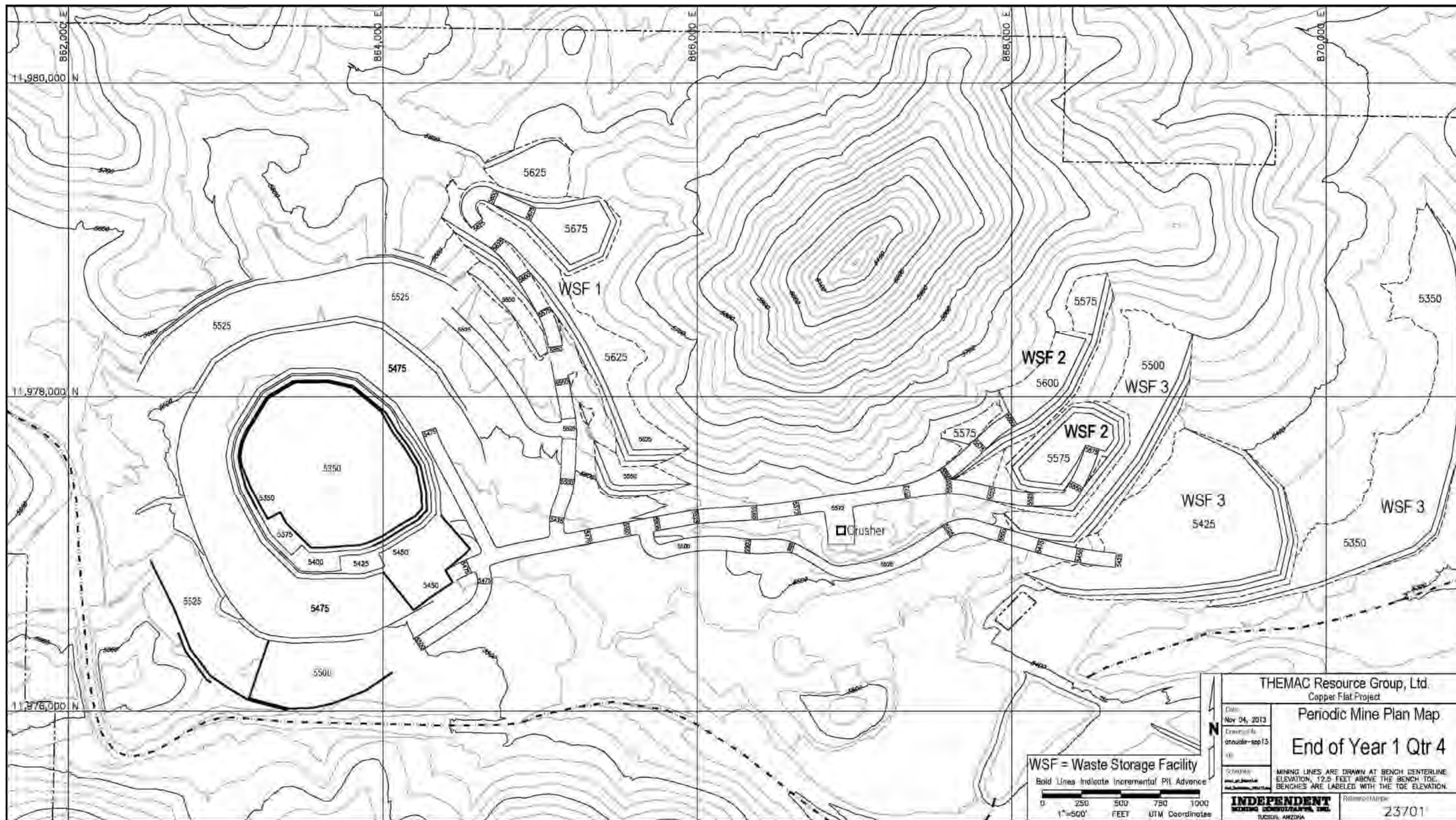
Figure 16-6: Periodic Mine Plan Map - End of Year 1 Q4
