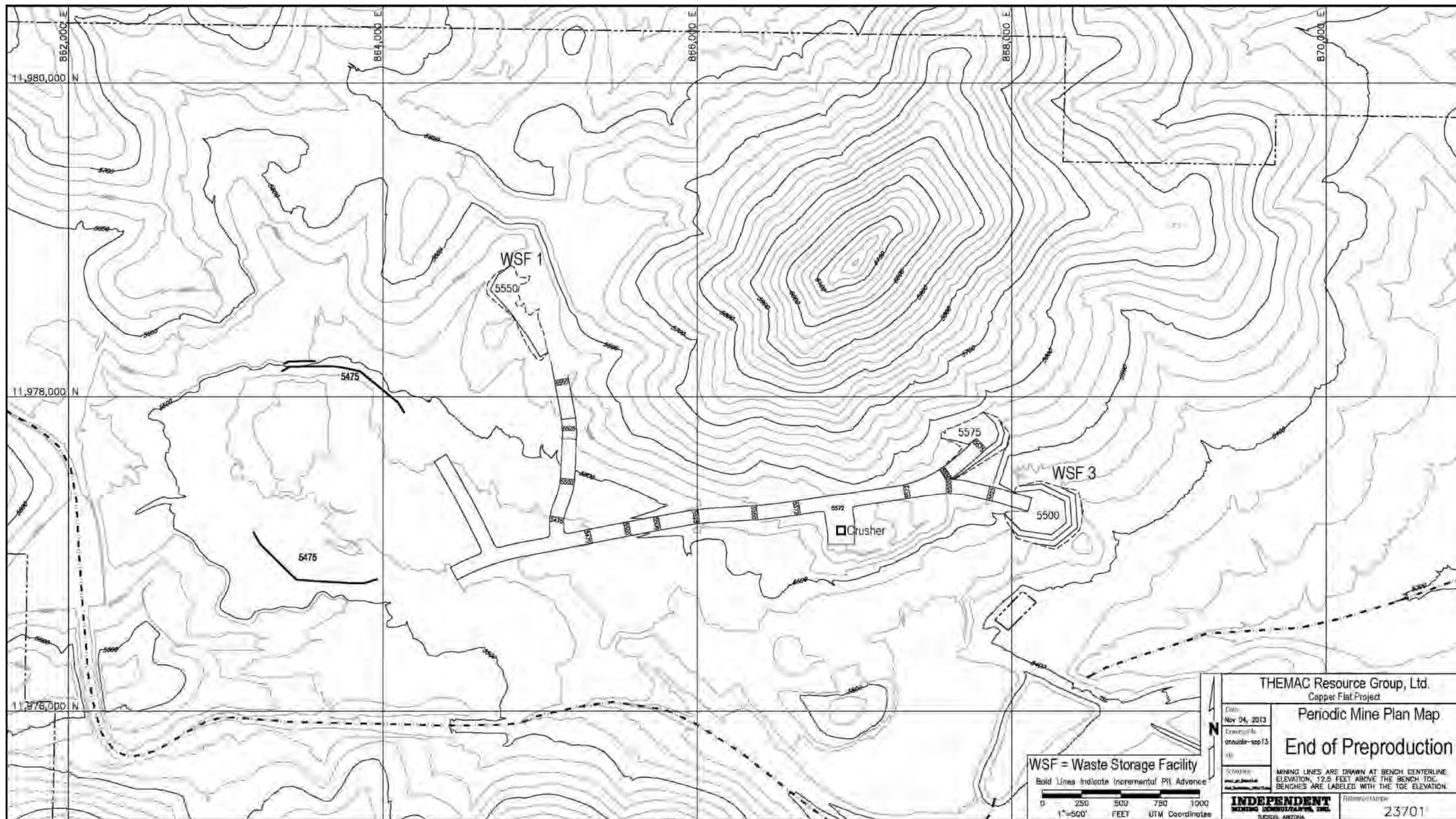
Figure 16-2: Periodic Mine Plan Map - End of Preproduction
