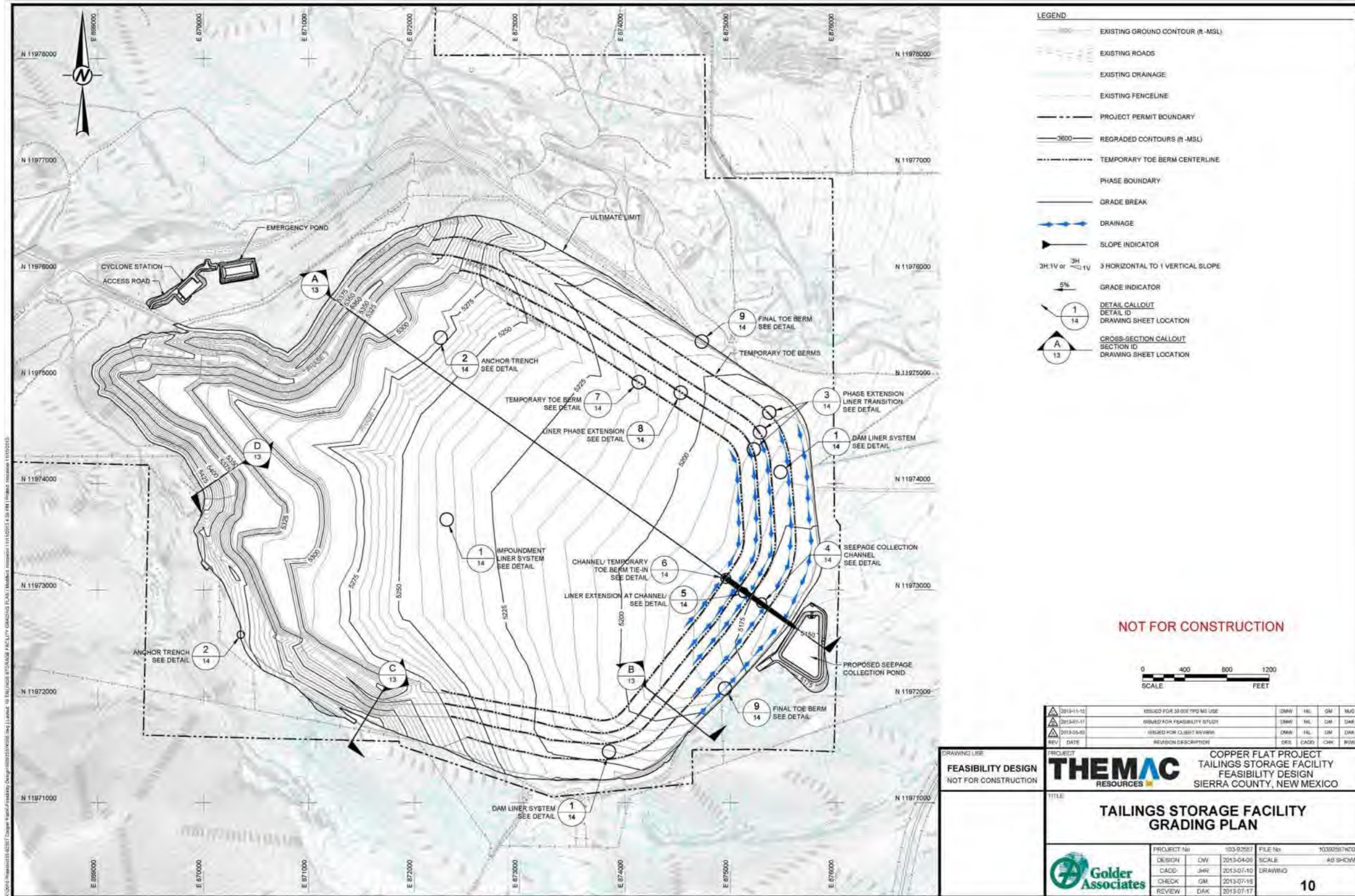
Figure 20-4: Tailings Storage Facility Grading Plan
