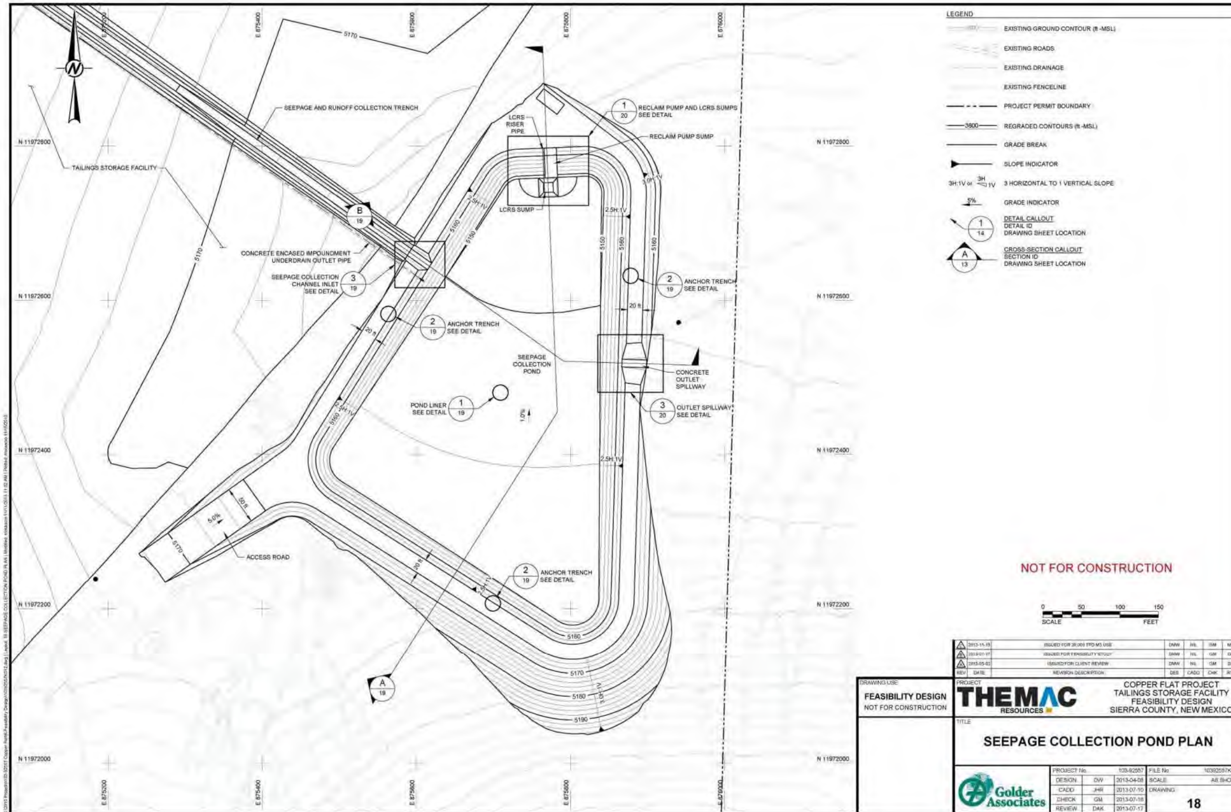
Figure 20-9: Seepage Collection Pond Plan
