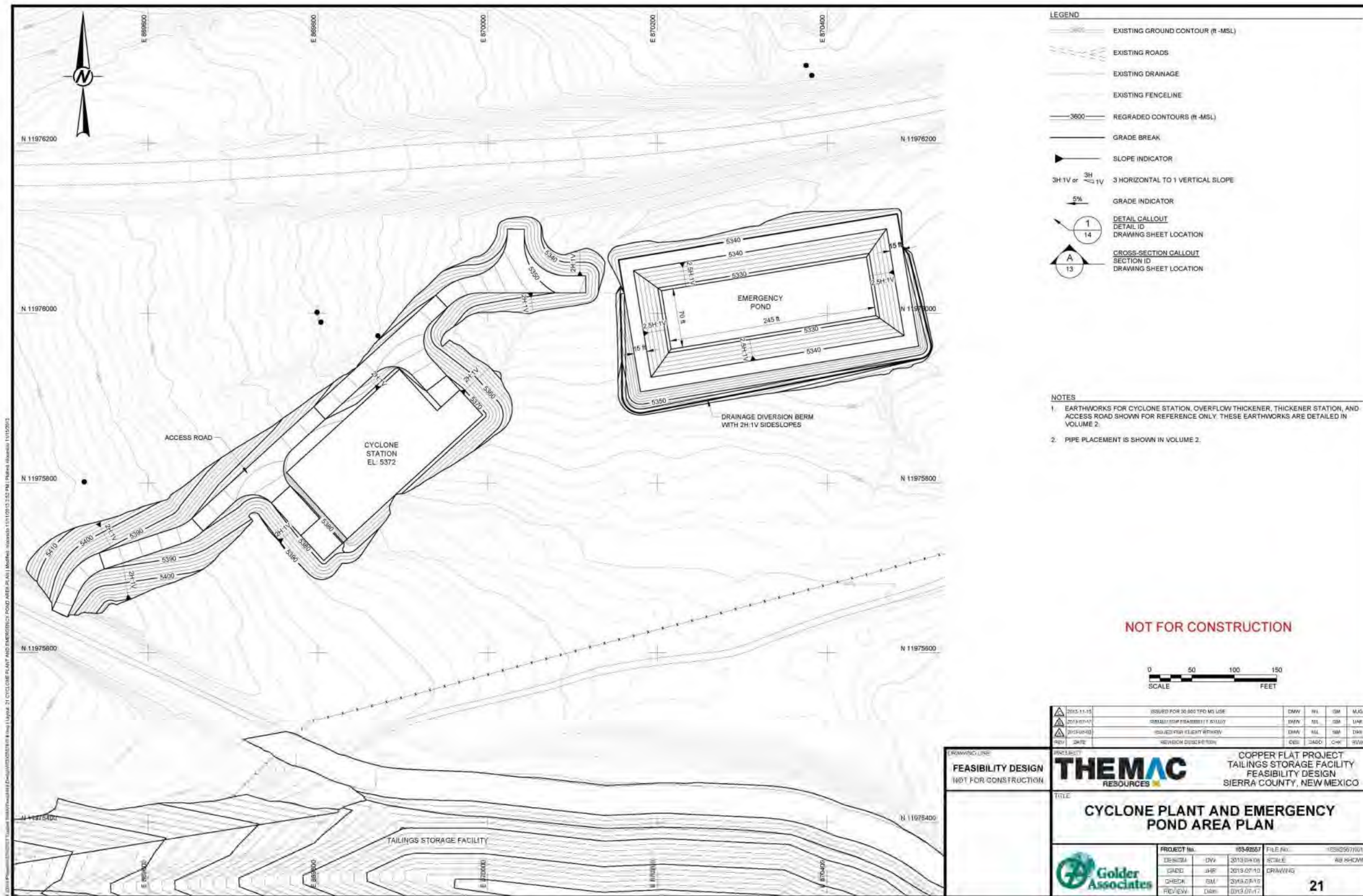
Figure 20-10: Cyclone Plant and Emergency Pond Area Plan
