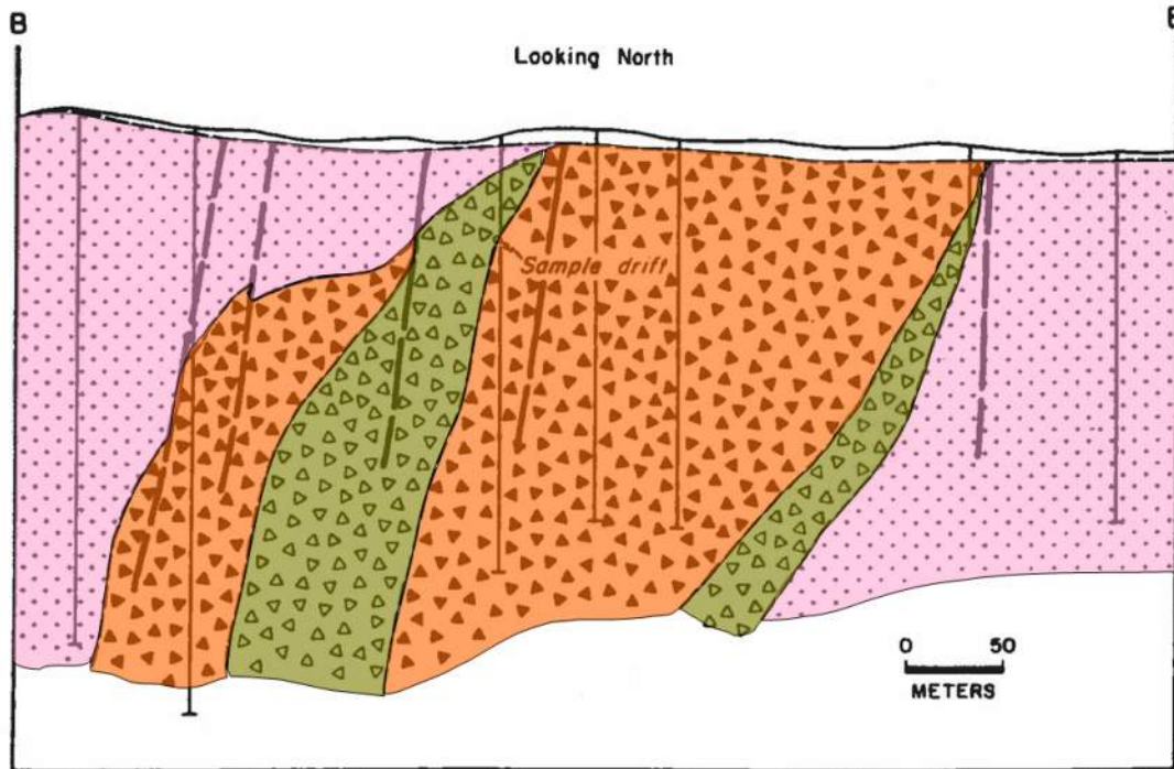
Figure 1-6: East-West Section Looking North, Dunn, 1982
