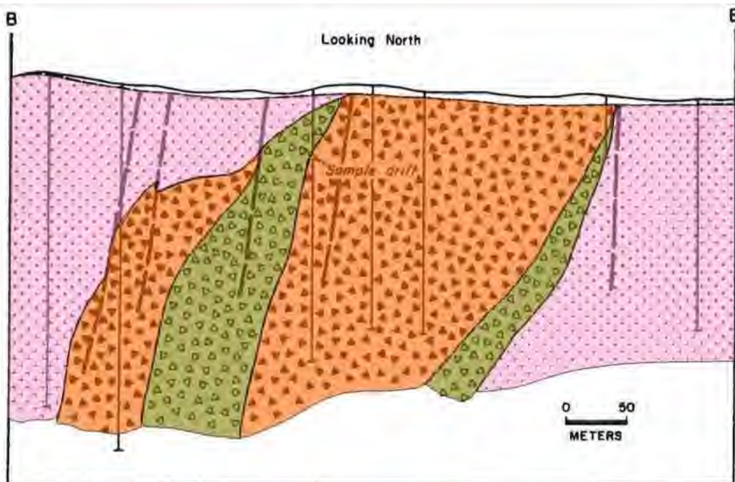
Figure 7-3: East-West Section Looking North, Dunn, 1982
