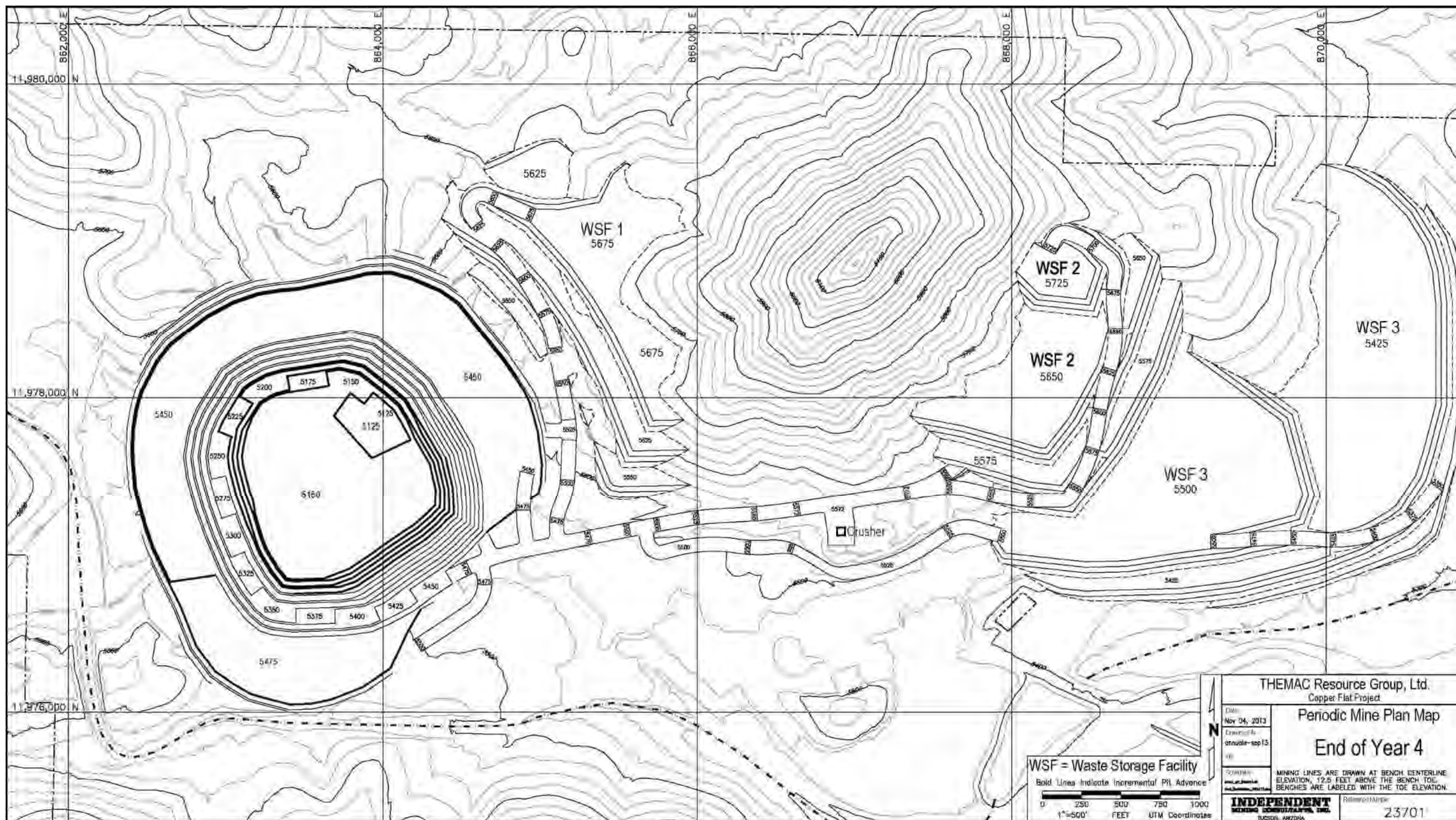
Figure 16-9: Periodic Mine Plan Map - End of Year 4
