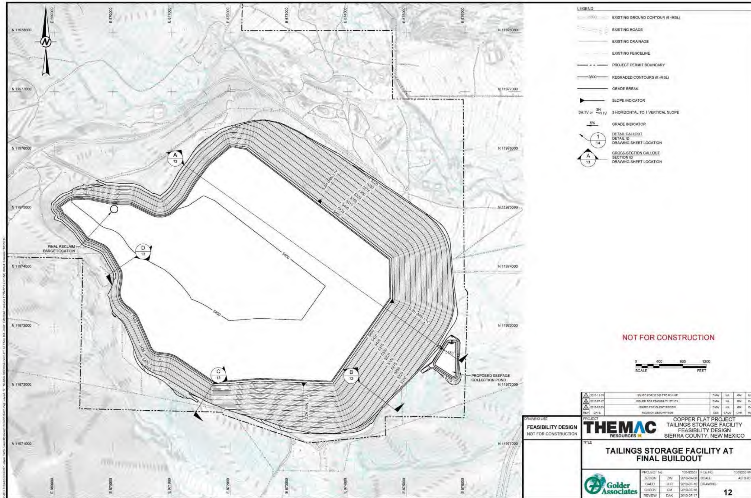
Figure 20-6: Tailings Storage Facility at Final Buildout
